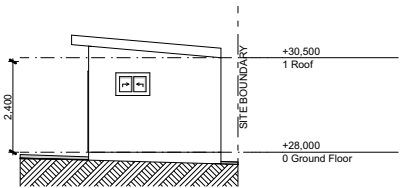
North Elevation 1:200
